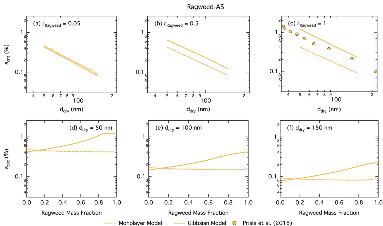
Fig. 11 Critical supersaturations calculated by using the monolayer and Gibbs models as a function of dry particle size for ragweed pollen mass fractions (a) 0.05; (b) 0.5; (c) 1 and as a function of ragweed pollen mass fraction for dry particle sizes (d) 50 nm; (e) 100 nm; and (f) 150 nm. Measured critical supersaturations as a function of pure ragweed pollen dry particle size from Prisle et al. 12 are also shown in panel (c).
