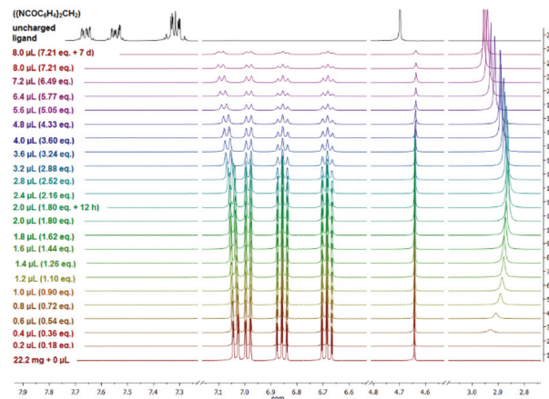
Fig. 4 Stacked 1 H NMR spectra (thf-d 8 ) of a titration experiment of [(\{NCOC_6H_4\}_2CH)K(thf)]_n ( 2 ) with water and a free uncharged ( \{NCOC_6H_4\}_2CH_2 ) ligand (black).
