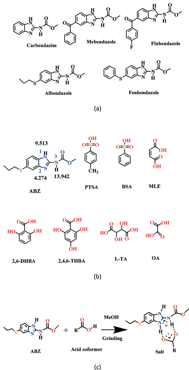
Scheme 1 (a) A few benzimidazole drugs. (b) Chemical structures of ABZ (along with their N pK_a values, will be discussed in later sections) and the coformers reported in this study. (c) Ionic synthon of ABZ with carboxylic acid in an R_2^2(8) motif.
