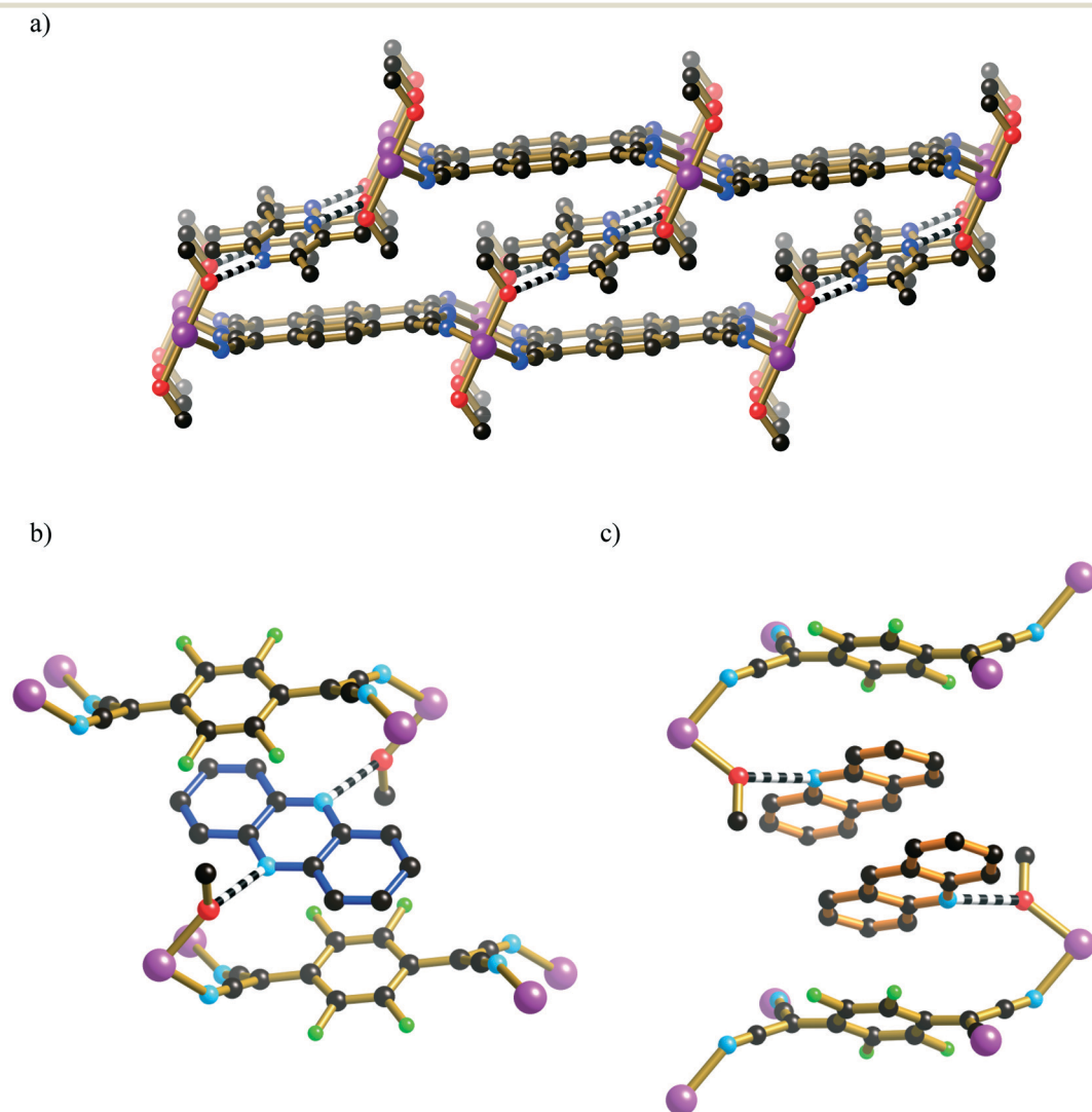
Fig. 3 a) The structure of [Zn(TCNQ)(MeOH) 2 ]·tmpyz (14) in which sheets are linked via H-bonding between coordinated MeOH ligands and tetramethylpyrazine units (H-bonds represented by striped connections). b) The structure of [Mn(F 4 TCNQ)(MeOH) 2 ]·phenazine (16) showing the H-bonding and aromatic interactions of the phenazine molecule. c) The H-bonding and stacking in [Mn(F 4 TCNQ)(MeOH) 2 ]·2-acridine (17).
