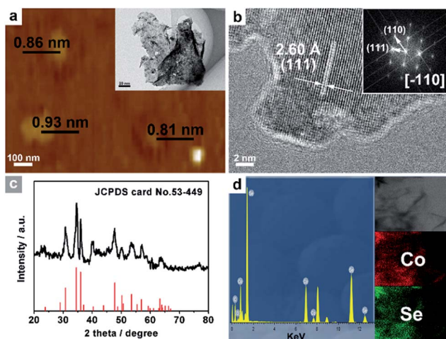
Fig. 5 (a) AFM image and TEM image (inset a), and (b) HRTEM images and the associated FFT pattern (inset b) of \text{CoSe}_2 UPNSs. (c) XRD pattern, (d) EDS spectrum and STEM-EDS elemental mapping images (inset d) of \text{CoSe}_2 UPNSs.
