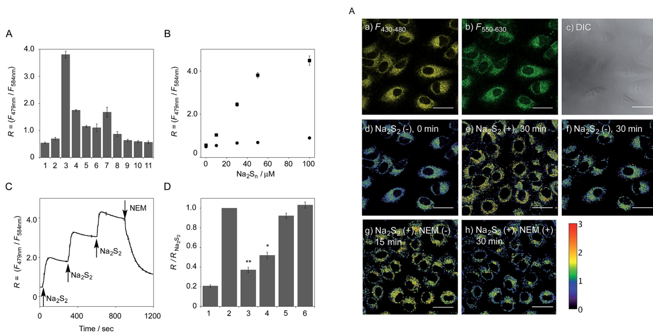
Fig. 3 (A) The ratio value ( R = F_{479\text{nm}}/F_{584\text{nm}} ) of 6 in the presence of various thiol species: (1) none, (2) Na 2 S (50 \mu\text{M} ), (3) Na 2 S 2 (50 \mu\text{M} ), (4) Na 2 S 4 (50 \mu\text{M} ), (5) CysSSH (NOC7 (50 \mu\text{M} ) + Na 2 S (50 \mu\text{M} ) + L-Cys (50 \mu\text{M} )), (6) GSSH (NOC7 (50 \mu\text{M} ) + Na 2 S (50 \mu\text{M} ) + GSH (50 \mu\text{M} )), (7) mixture of NaOCl (50 \mu\text{M} ) and Na 2 S (50 \mu\text{M} ) in 0.1 M NaOH, (8) mixture of NaOCl (50 \mu\text{M} ) and Na 2 S (50 \mu\text{M} ) in 50 mM HEPES buffer (pH 7.4), (9) GSH (5 mM), (10) L-Cys (1 mM), (11) cystine (0.5 mM). Measurement conditions: [6] = 5 \mu\text{M} in 50 mM HEPES, 10 mM NaCl, 1 mM MgSO 4 , 0.4% Tween, pH 7.4, 25 °C. \lambda_{\text{ex}} = 410 nm. n = 3. (B) Change in the fluorescence intensity ratio of 6 (5 \mu\text{M} ) upon addition of Na 2 S 2 (0–100 \mu\text{M} , ■) and Na 2 S (0–100 \mu\text{M} , ●). n = 3. (C) Time-trace plot of the ratio value ( R = F_{479\text{nm}}/F_{584\text{nm}} ) of 6 (5 \mu\text{M} ) upon addition of Na 2 S 2 (30 \mu\text{M} at 30, 300, and 600 s) and N-ethylmaleimide (NEM, 500 \mu\text{M} at 900 s), n = 3. (D) The reverse change of the ratio value ( R = F_{479\text{nm}}/F_{584\text{nm}} ) of 6 induced by the reactive species. Each bar represents R value of: (1) 6 (5 \mu\text{M} ), (2) the hydropersulfide adduct of 6 (5 \mu\text{M} ) with Na 2 S 2 (50 \mu\text{M} ), (3) the adduct + NaOCl (100 \mu\text{M} ), (4) the adduct + NEM (200 \mu\text{M} ), (5) the adduct + GSH (5 mM), and (6) the adduct + L-Cys (1 mM). Measurement conditions: 50 mM HEPES, 10 mM NaCl, 1 mM MgSO 4 , 0.4% Tween, pH 7.4, 25 °C. \lambda_{\text{ex}} = 410 nm. n = 3; * P < 0.05, ** P < 0.01 vs. hydropersulfide adduct of 6 with Na 2 S 2 (lane 2).
