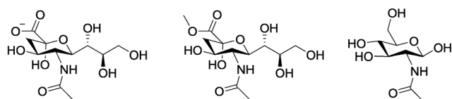
Fig. 9 Structures of sialic acid (left), the corresponding methyl ester (centre) and N -acetyl- \text{D} -glucosamine (right).
