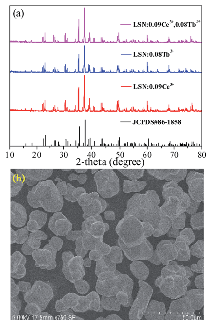
Fig. 1 (a) Powder XRD patterns of La 0.91 Si 3 N 5 :0.09Ce 3+ , La 0.92 Si 3 N 5 :0.08Tb 3+ and La 0.83 Si 3 N 5 :0.09Ce 3+ , 0.08Tb 3+ phosphors. The standard data of CeSi 3 N 5 (JCPDS No. 86-1858) is shown as a reference. (b) SEM image of the as-prepared La 0.83 Si 3 N 5 :0.09Ce 3+ , 0.08Tb 3+ phosphor.
