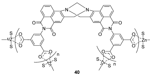
Fig. 21 Structures of the fluorescent chemosensors 39a–c and 40 .
