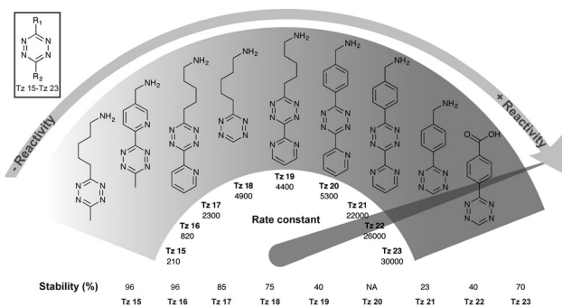
Fig. 16 Second order rate constants of selected tetrazines with TCO in PBS at 37^\circ\text{C} and corresponding stability assessed in PBS at 37^\circ\text{C} for 10 h. NA, not assessed. 40
