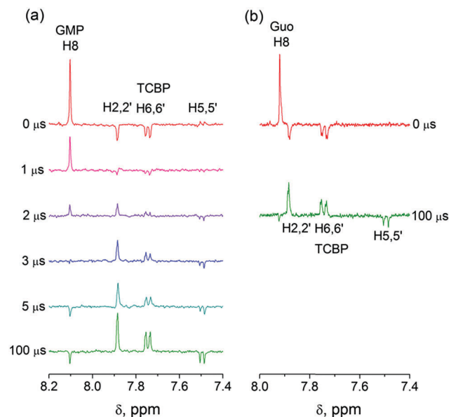
Fig. 1 (a) 1 H CIDNP spectra, detected in the photoreaction of 2 mM 3,3',4,4'-tercarboxy benzophenone and 20 mM guanosine-5'-monophosphate in 50 mM sodium phosphate buffer at pH 6.9 at variable time delays after the laser pulse. The delays are ascending from 0 (top) to 100 μs (bottom spectrum). (b) 1 H CIDNP spectra detected in the photoreaction of 2 mM 3,3',4,4'-tercarboxy benzophenone and 2 mM guanosine in 50 mM sodium phosphate buffer at pH 6.9. The upper spectrum was taken immediately after the laser pulse, and the lower spectrum at 100 μs after the laser pulse.
