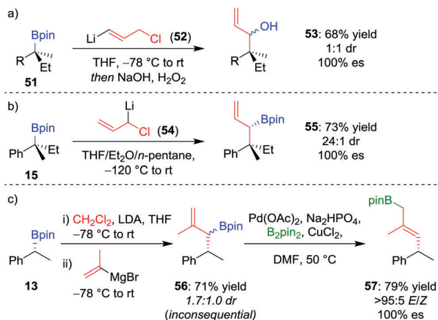
Scheme 10 Three-carbon homologies of enantioenriched boronic esters, and the palladium-catalyzed 1,3-borotropic shift. R = \text{CH}_2\text{CH}_2\text{Ph} .
