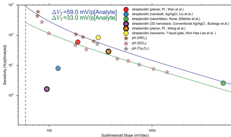
Fig. 9 The relationship between Sensitivity and subthreshold slope, for measurements obtained within the subthreshold region. Both streptavidin sensing 26,28,32,49,70,107 (●) and pH sensing data (★) 18,38,44,183–190 are shown. For pH sensing, consistent surface potential changes are observed for a given oxide, resulting in the ability to predict Sensitivity accurately using eqn (9). In contrast, for biosensing, eqn (9) was insufficient to accurately predict Sensitivity, indicative of significant surface potential variation per 10-fold increase in streptavidin concentration. All biosensing and pH sensing measurements were performed using a liquid top-gate, with the exception of the biosensing measurements of Elfström et al. which utilised a fixed back-gate voltage with no liquid top-gate. For streptavidin-sensing data, the device geometry, liquid top-gate reference electrode material and authors, respectively, are shown in parenthesis within the legend. Dielectrics show a characteristic shift in threshold voltage per change in pH unit that is ~33 mV per pH for SiO 2 and ~59 mV per pH for HfO 2 . Curves calculated using eqn (9) for a threshold voltage shift per 10 fold increase in analyte concentration of 33 mV and 59 mV are shown using solid lines. The dashed line indicates the theoretical lower limit of the subthreshold slope at room temperature of 59 mV dec -1 available to classical FETs. Details of method used to obtain the data and a replot of the same data but on a linear x-axis can be found in ESI 7.6.†
