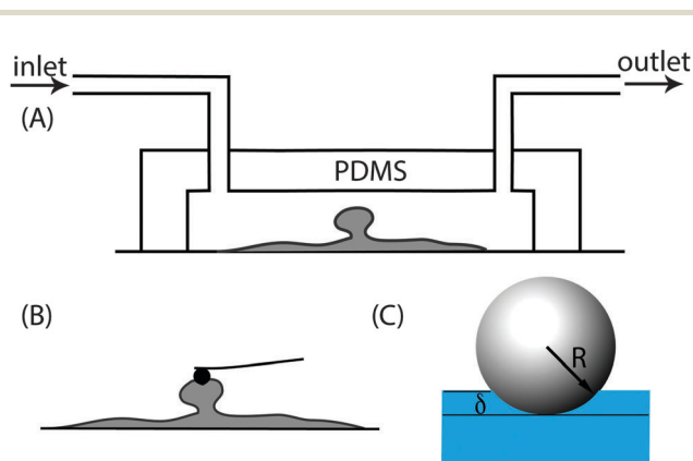
Fig. 1 (A) Experimental set up of the flow cell showing the biofilm growing on the glass surface of the chamber. (B) AFM cantilever with a spherical polystyrene tip of radius 5 \mu\text{m} was used to probe the surface of the biofilm. (C) The Young's modulus was measured from the indentation depth for a given force.
