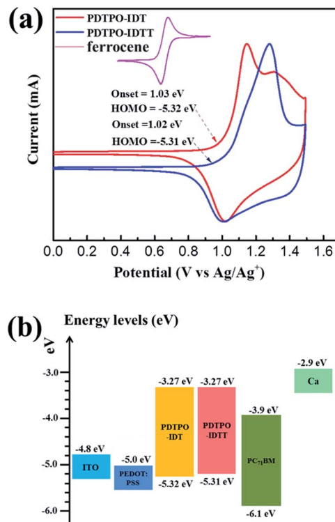
Fig. 2 (a) The electrochemical cyclic voltammetry measurements of PDTPO-IDT and PDTPO-IDTT thin film coated on the platinum electrode in acetonitrile solution containing 0.1 M n\text{-Bu}_4\text{NPF}_6 at a scan rate of 100 \text{ mV s}^{-1} . (b) Schematic energy level diagram of all components used in conventional devices.
