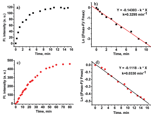
Fig. 7 (a) Reaction-time profiles of CHMC-thiol ( 5.0 \mu\text{M} ) in the presence of 100 \mu\text{M} Cys ( \blacksquare ) at 680 \text{ nm} ; (b) pseudo-first-order kinetic plot of the reaction of the probe CHMC-thiol ( 5 \mu\text{M} ) with Cys ( 100 \mu\text{M} ) at 680 \text{ nm} in pH 7.4, 25 \text{ mM} PBS. Slope = 0.3295 \text{ min}^{-1} ; (c) reaction-time profiles of CHMC-thiol ( 5.0 \mu\text{M} ) in the presence of 500 \mu\text{M} Cys ( \blacksquare ) at 625 \text{ nm} ; (d) pseudo-first-order kinetic plot of the reaction of the probe CHMC-thiol ( 5 \mu\text{M} ) with Cys ( 500 \mu\text{M} ) at 625 \text{ nm} in pH 7.4, 25 \text{ mM} PBS. Slope = 0.0330 \text{ min}^{-1} .
