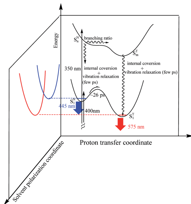
Fig. 8 The ES IPT of 3-HTCA in the S 1 N and S 1 T states. The 3D plot contains the proton transfer coordinate and solvent polarization coordinate. The latter is where the solvent induced barrier is introduced during ES IPT in the lowest lying states. This is due to different equilibrium polarization between S 1 N and S 1 T , which is presented by its coupling with the solvent polarity induced barrier along the solvent polarization coordinate.
