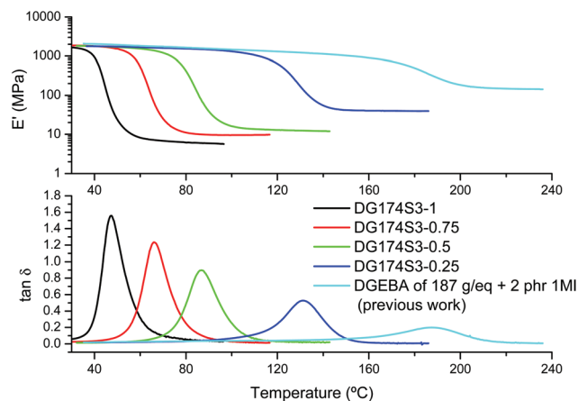
Fig. 6 DMA analysis of DG174S3- r formulations in comparison with a neat epoxy homopolymer from a previous work. 27
