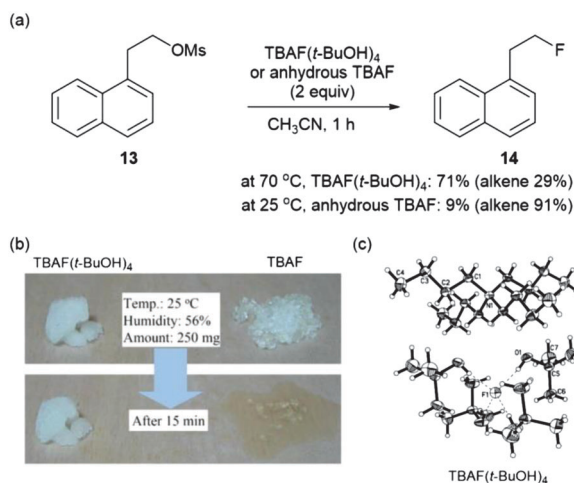
Fig. 4 (a) Comparison of the reactivity and selectivity of TBAF( t -BuOH) 4 and anhydrous TBAF in a nucleophilic fluorination reaction. (b) Reduced hygroscopicity of TBAF( t -BuOH) 4 . (c) X-ray crystal structure of TBAF( t -BuOH) 4 .
