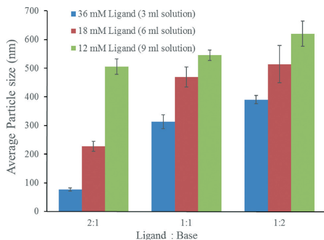
Fig. 3 Average particle size of 1b-S after 0.5 h by altering the concentration of H 2 b 2 ccppm and the ligand to base ratio from 2:1 to 1:1 and 1:2.
