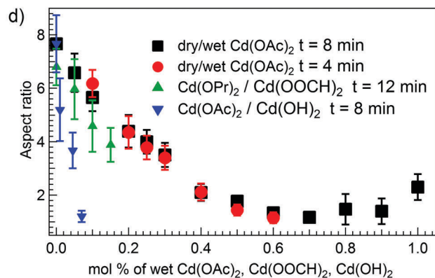
Fig. 2 TEM images of samples (a) NPL-1, (b) NPL-6, (c) and NPL-10 illustrating the aspect ratio control. (d) Plot of the CdSe NPL aspect ratio versus the molar percentage of Cd(OAc) 2 ·2H 2 O, Cd(OOCH) 2 , and Cd(OH) 2 precursors, respectively.
