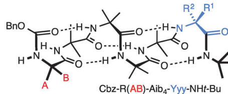
(b) Varying the C terminus of \text{Cbz-R(AB)-Aib}_4\text{-Yyy-NHt-Bu} .
