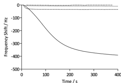
Fig. 3 Frequency responses of protein binding to QCM sensors. Anti-biotin F_{ab} binding to biotin-derivatized pAAc surface (—); anti-biotin F_{ab} binding to biotin-derivatized carboxyl-terminated SAM surface (---); anti-biotin F_{ab} binding to deactivated pAAc surface (···); lysozyme binding to biotin-derivatized pAAc surface (·-·). Sample concentrations: 25 \mu\text{g mL}^{-1} ; flow rate: 25 \mu\text{L min}^{-1} .
