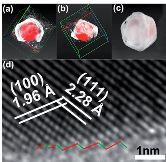
Fig. 3 3D reconstruction images (a and b) viewed from distinct angles, surface-rendered view reconstructed by the HAADF-STEM tomography (c) of an OM-YS Au@AgPd NP, HRTEM image (d) of the edge of a curved region of an OM-YS Au@AgPd NP (the inset in Fig. 2a).
