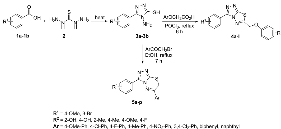
Scheme 1 Synthesis of triazolothiadiazoles ( 4a–l ) and triazolothiadiazines ( 5a–p ).
