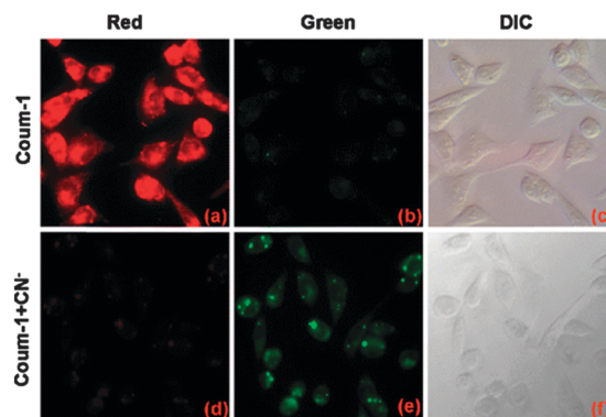
Fig. 29 Top: structure and chemodosimetric reaction of Coum-1 with \text{CN}^- . Bottom: images of HeLa cells incubated with Coum-1 with and without \text{CN}^- ; (a, d) red channel (b, e) green channel and (c, f) brightfield differential interference contrast (DIC). Image reproduced with permission. 175
