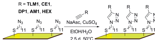
Scheme 2 Surface attachment of organic molecules via "click" chemistry (NaAsc = sodium ascorbate).
