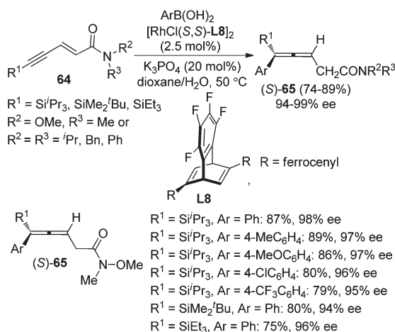
Scheme 22 Rh-catalyzed asymmetric 1,6-addition of arylboronic acids to enynamides.
