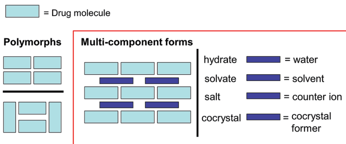
Fig. 9 Schematic of the characteristics of polymorphs and multicomponent systems. Cocrystals represent a sub-set of the multicomponent group, frequently that characterised by the requirement that the components be neutral and solid at room temperature.
