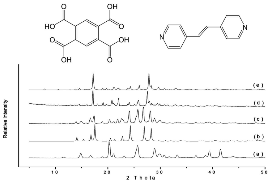
Fig. 15 Demonstration of the enhanced kinetics of cocrystal formation upon addition of a few drops of methanol to the grinding jar. PXRD patterns for (a) tetracarboxylic acid, (b) bipryridyl, (c) outcome of neat grinding for 60 minutes (as the sum of the reactants), (d) the product obtained when a few drops of methanol are added and (e) the simulated pattern for the cocrystal.
