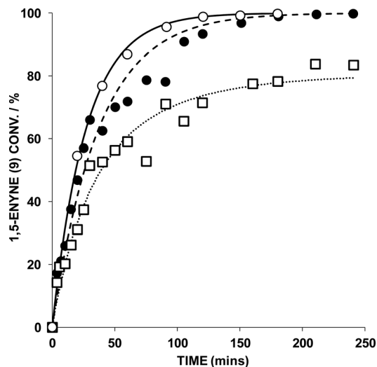
Fig. 4 Effect of 1,5-enyne concentration [9] in a reaction mediated by AuBr 2 (N-phthal)(I t Pe) (1 mol%), AgOTf (1 mol%), in DCE at 25 °C (key: ○ = 0.1 M 9 ; ● = 0.2 M 9 ; □ = 0.5 M 9 ). 1,5-Enyne conversion monitored by GC analysis – each sample point was quenched by addition of ( n -Bu) 4 NBr. The kinetic curves were fitted using Dynafit™.
