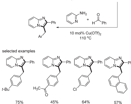
Scheme 63 Four-component reaction for the synthesis of imidazo[1,2-a]pyridines.
