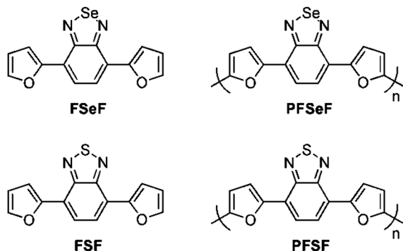
Scheme 1 Chemical structures of FSeF , FSF monomers and their corresponding polymers PPFSeF and PPFSF .
