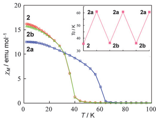
Fig. 6 Temperature dependences of \chi_M for the initial form 2 ( \circ ), the dehydrated form 2a ( \square ) and the rehydrated form 2b ( \triangle ) in an applied dc field of 500 Oe. The insert shows the reversible T_C switching by dehydration/hydration treatments (red/blue arrows, respectively).
