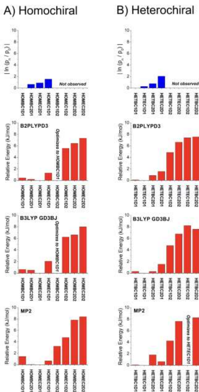
Figure 6 A graphical representation of the relative isomer energies reported in Table 1 for calculations with the def2TZVP basis set is shown. The three quantum chemistry methods are B2PPLYPD3, B3LYP GD3BJ, and MP2. In some cases, the geometry optimization collapsed into the lower energy geometry with different dihedral angle about the O---O axis of the hydrogen bond and these cases are indicated in the figure. An analogous figure using the 6-311++G(d,p) basis set is available in the supporting information.
