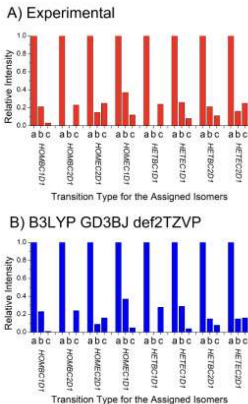
Figure 11 The top panel shows the experimental determination of the relative intensities of the a-, b-, and c-type rotational spectrum components for the 8 chiral tag complexes identified in this work. These relative intensities are governed by the ratio of the squares of the a-, b-, and c-components of the dipole moment vector represented in the principal axis system. The relative intensities of the square of the dipole moment components in the B3LYP GD3BJ def2TZVP calculations are shown in the bottom panel.
