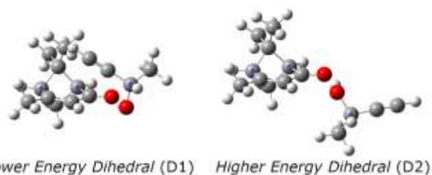
Figure 1 The structural characterization of the lowest energy isomers of the 1:1 complexes formed between verbenone and butynol is illustrated. The two hydrogen bond positions are shown in the top panel (A). Most quantum chemistry methods identify two equilibrium geometries for the dihedral angle around the O---O axis of the hydrogen bond as shown in panel (B). The structures shown in this figure are equilibrium geometries from the B3LYP GD3BJ def2TZVP calculation set.
