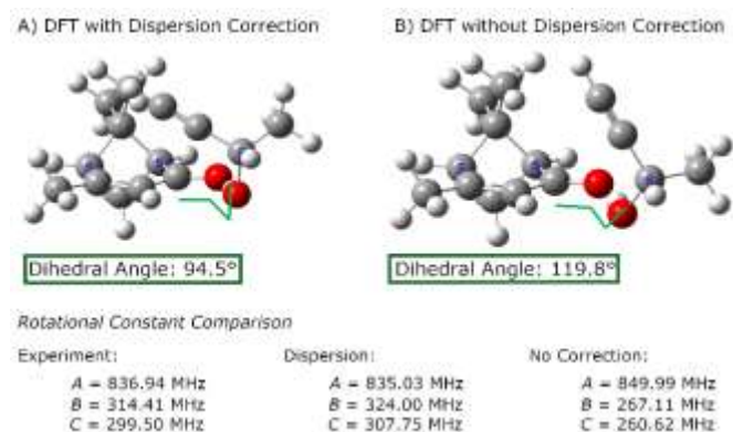
Figure 3 This figure illustrates the need to include dispersion corrections in the geometry optimization calculations of the verbenone-butynol chiral tag complexes. The dispersion interactions are important in determining the dihedral angle about the O---O axis of the hydrogen bond formed between the hydroxyl group of butynol and the carbonyl group of verbenone. The DFT calculation without dispersion correction, shown to the right in (B), has poor agreement between the experimental rotational constants and those calculated from the equilibrium geometry. Calculations were performed with B3LYP and the def2TZVP basis set and GD3BJ dispersion correction.
