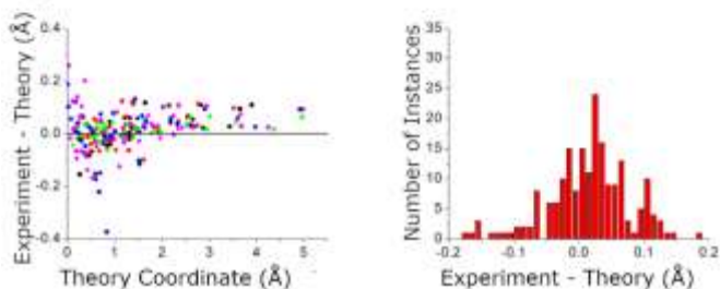
Figure 9 The accuracy of the quantum chemistry structures is benchmarked using the carbon atom coordinates – in the principal axis system for molecular rotation – obtained from the Kraitchman analysis. The scatter plot shows the difference in the absolute values of these coordinates (coordinate signs are unavailable from the spectroscopic analysis) as a function of the size of the coordinate. The coordinates come from the 5 structures that were measured with ^{13}\text{C} -sensitivity: HOMEC2D1 (black), HOMBC2D1 (blue), HOMBC1D1 (magenta), HETEC1D1 (red), and HETBC1D1 (green). The figure for calculations with the 6-311++G(d,p) basis set is shown in the supporting information.
