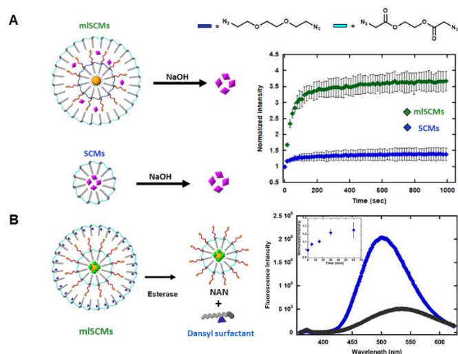
Figure 2. Fluorometric analysis of various mISCM constructs. A) Fluorometric analysis of 5-TAMRA release from SCMs vs gold encapsulated mISCMs in the presence of sodium hydroxide (ex. 557 nm, em. 583 nm). An enhanced release profile is observed from mISCMs due to quenching of the 5-TAMRA in close proximity to the gold nanoparticles. B) Analysis of breakdown of the outer layer of an mISCM built with dansyl modified surfactant (ex. 330 nm, em. 360–625 nm). A blueshift and decrease in intensity is observed. Inset: Analysis of release of fluorescein from the inner layer of a mISCMs (ex. 488 nm, em. 508 nm).
