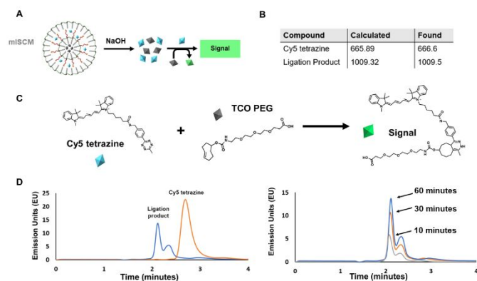
Figure 3. Chemical reactions gated at the nanoscale A) Schematic representation of stimuli-responsive cargo release from distinct mISCM layers that results in signal (product formation shown in C). B) Mass spectrometry analysis of the products of the release of cargo from individual layers of the mISCMs. C) Trans-cyclooctene – tetrazine ligation between cyanine5 tetrazine and trans-cyclooctene PEG. D) HPLC assay showing TCO – tetrazine ligation product formation after release from mISCMs (left). Initial release profiles of cyanine5 tetrazine from the outer layer of an mISCM after release of TCO. Ligated product formation is observed over a 30-minute time course (right).
