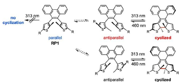
Fig. 14 Reversible photocyclization processes of atropisomeric dithienylethenes (RP1). Reversible switching of a conformational isomer (antiparallel rotamer only) upon irradiation.
