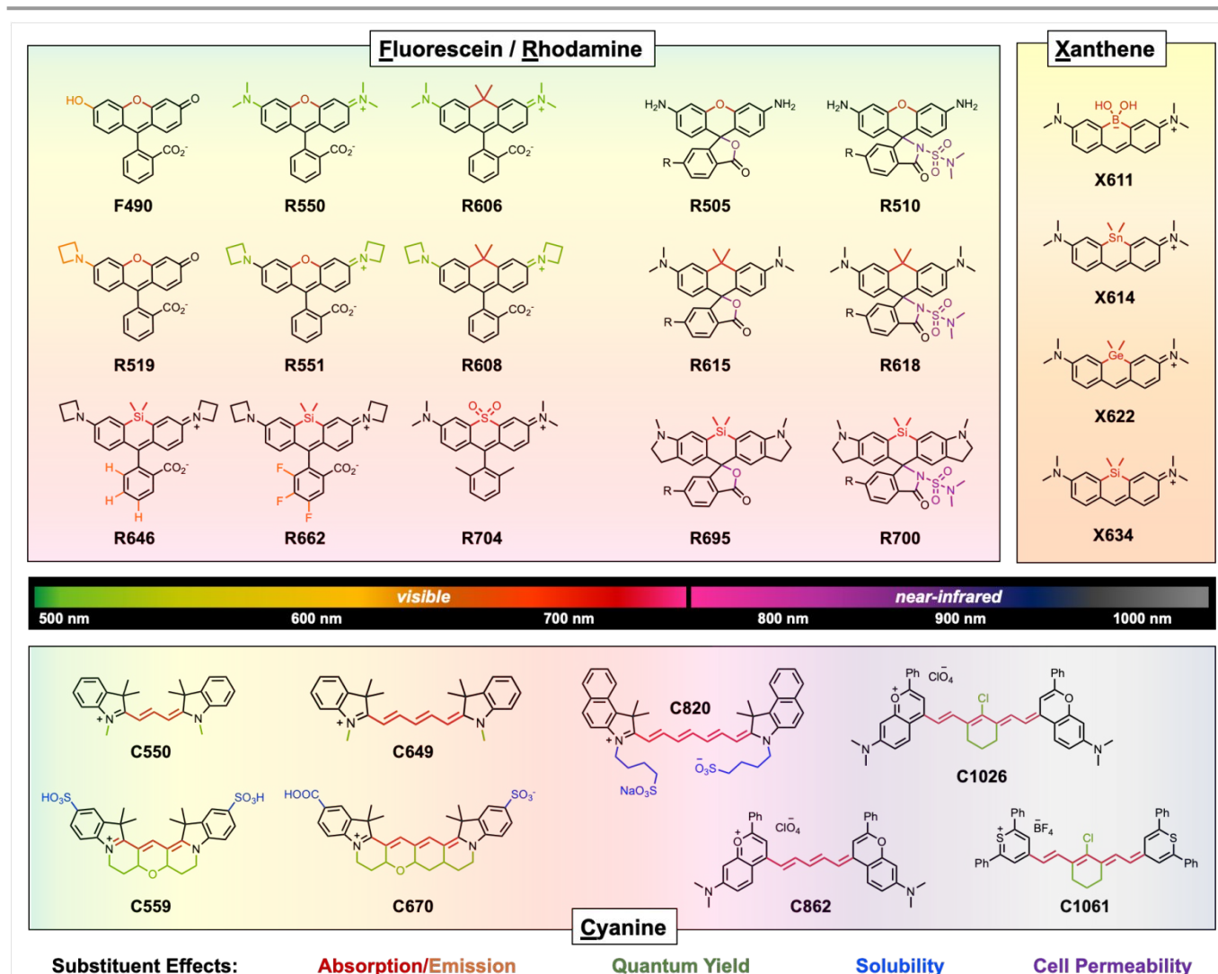
Fig. 5 Structure-photophysical relationship chart of visible and NIR dyes. From ‘top to down’ or ‘left to right’ within the core, increase in absorption and emission (red-xanthenes substituent /orange-phenyl ring substituent), increase in quantum yield (green), increase in cell permeability (purple), and increase in solubility in water (blue). Compound naming consist of first letter (F, R, X, or C) of core scaffold and its maximum absorption. R group is HaloTag ligand.
