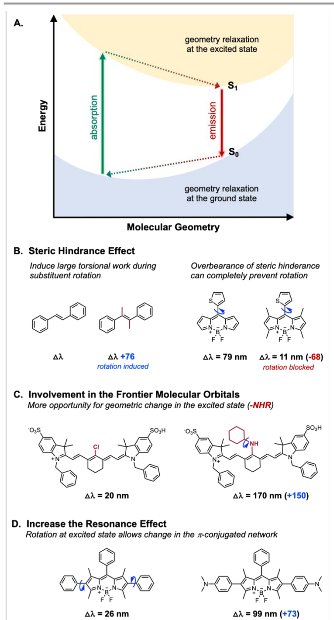
Fig. 6 Choice of rotating substituent on Stokes shift ( \Delta\lambda ). A. Schematic illustration of absorption and emission process in fluorophore, B. Steric hindrance effect on Stokes shift, C. Effect of frontier molecular orbital in Stokes shift, and D. Resonance effect on Stokes shift.
