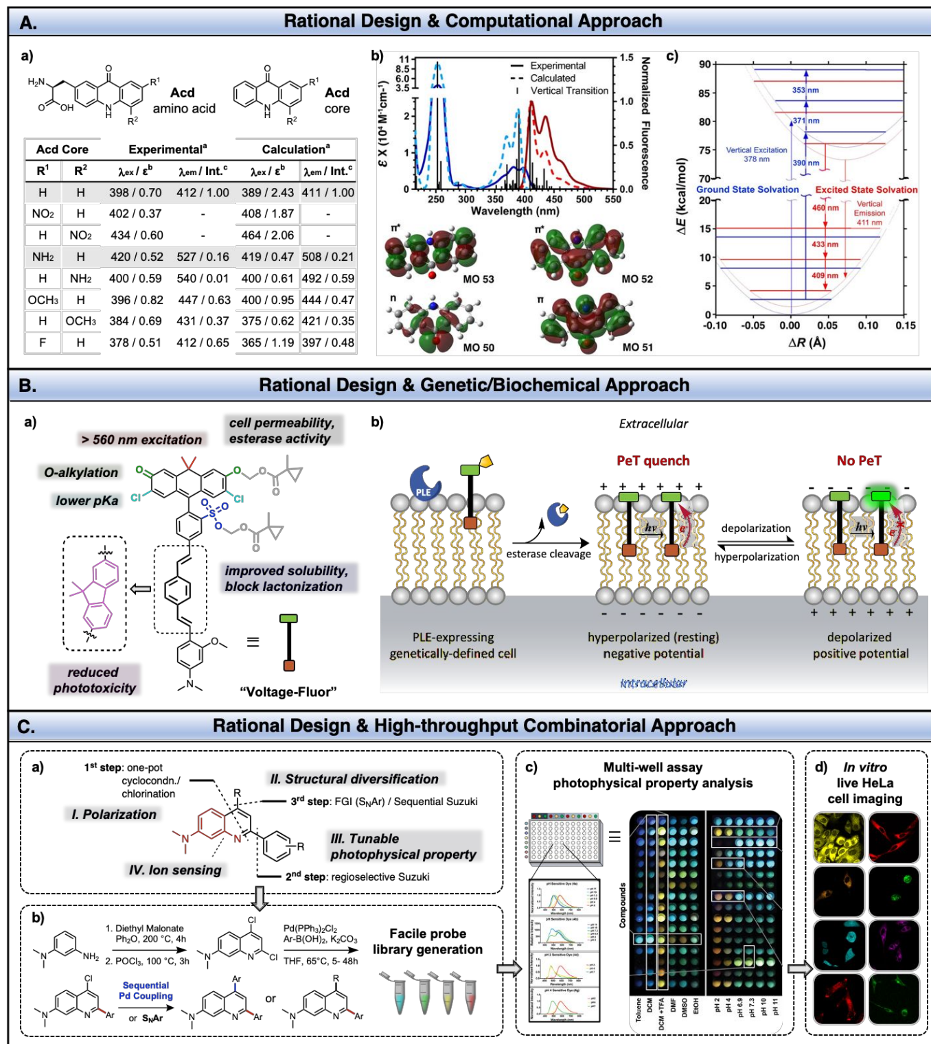
Fig. 15 A. Design and photophysical properties of acridonylalanine (Acd) based probe. a) Calculated and experimental values of Acid core derivatives. a Lowest energy absorption and highest intensity emission values. b Extinction coefficients ( \epsilon ) reported as 10^4 \text{ M}^{-1} \text{ cm}^{-1} . c Normalized emission intensity (Int.) of the highest emission of acridone ( R^1, R^2 = \text{H} ). b) Franck-Condon corrected spectra with molecular orbitals (MOs) involved in the n \rightarrow \pi^* and \pi \rightarrow \pi^* transitions of acridone ( R^1, R^2 = \text{H} ). c) Jablonski diagram of frozen ground or excited state solvation. Adapted from ref 96. Copyright (2018) John Wiley & Sons, Ltd. B. a) Rational design of Voltage-Fluor . b) Scheme of voltage-sensitive fluorescence mechanism is shown. Membrane labelling of Voltage-Fluor to porcine liver esterase (PLE)-expressing cells. At rest, negative membrane potential (hyperpolarized) enhances PeT quenching and diminishing fluorescence. Upon depolarization, the positive membrane potential reduces PeT quenching, resulting in enhanced fluorescence. C. a) Modularity and b) synthesis of dimethylamino quinoline ( DMAQ ) dyes. Stream-line probe discovery from scaffold design to c) multi-well plate reader analysis followed by d) live cell imaging. Specific examples of applications of these fluorophores are shown in Fig. 16. Adapted from ref 34. Copyright (2019) American Chemical Society.
