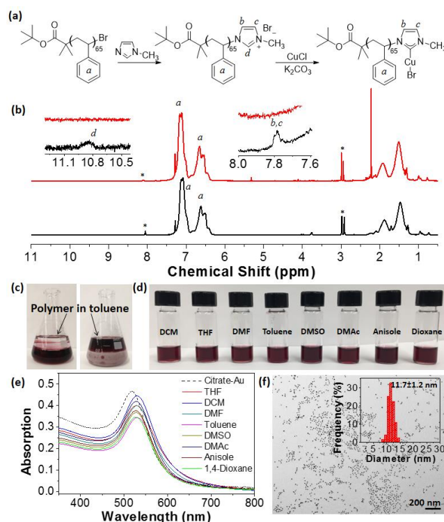
Figure 1. (a) Synthesis of \text{PS}_{65}\text{-NHC-Cu(I)} using end group functionalization to convert Br to NHC-Cu(I). (b) ^1\text{H} NMR spectra of \text{PS}_{65}\text{-Im} (black, bottom) and \text{PS}_{65}\text{-NHC-Cu(I)} (red, top) measured in d\text{-CHCl}_3 . *: residual DMF. (c) Images showing the transfer of citrate-capped AuNPs in water (bottom layer) to toluene (top layer) using \text{PS}_{65}\text{-NHC-Cu(I)} . (d) Images showing the dispersion of \text{PS}_{65}\text{-NHC} modified AuNPs in various solvents. (e) UV-vis spectra showing the SPR absorption of AuNPs in various solvents. (f) TEM image of \text{PS}_{65}\text{-NHC-Au} in THF. The inset shows the average size of AuNPs.
