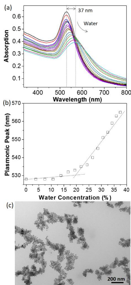
Figure 2. (a) UV-vis spectra of PS 65 -NHC modified AuNPs in THF when titrating with water. The spectra were collected by adding 80 \mu L of water each time into 2 mL of the THF solution of AuNPs. (b) Plotting the plasmonic peak of PS 65 -NHC modified AuNPs as a function of water concentration to determine the critical water concentration. (c) TEM image of PS 65 -NHC modified AuNPs in THF/water (1:1 vol) mixture.
