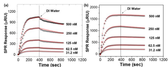
Figure 6. SPR traces showing the binding kinetics of (a) PMEO 2 MA 125 -NHC-Cu(I) and (b) PMEO 2 MA 174 -SH to Au. After the flow of polymer solution, the DI water was flowed over the Au sensor to trace the dissociation. The thin red lines are the fit curves of the kinetic data.
