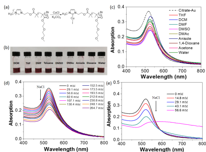
Figure 5. (a) Synthesis of PMEO 2 MA 125 -NHC-Cu(I) using an imidazole-containing ATRP initiator. (b) Image showing solutions of PMEO 2 MA 125 -NHC-Au in various organic solvents and water. (c) UV-vis spectra showing the SPR peaks of AuNPs dispersed in various solvents. (d,e) Titration experiments showing the stability of PMEO 2 MA 125 -NHC-Au (d) and citrate-capped AuNPs (e) upon addition of 1 M NaCl.
