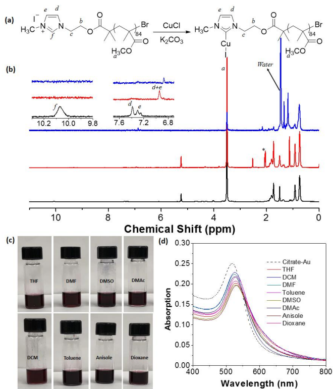
Figure 4. (a) Synthesis of PMMA 85 -NHC-Cu(I) using an imidazole-containing ATRP initiator. (b) 1 H NMR spectra of PMMA 85 -Im (black, bottom), PMMA 85 -NHC-Cu(I) (red, middle) and PMMA 85 -NHC-Au (blue, top) in CD 2 Cl 2 . (c) Images showing PMMA 85 -NHC-Au dispersed in various organic solvents. (d) UV-vis spectra showing the SPR absorption of PMMA 85 -NHC-Au in various solvents.
