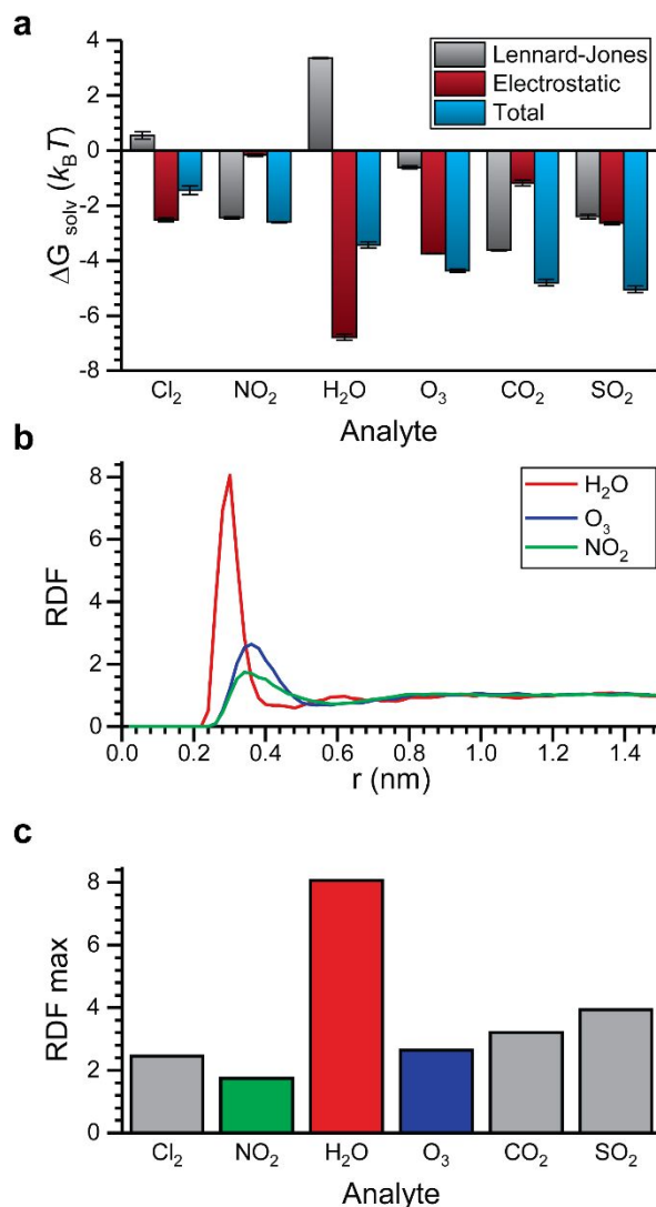
Figure 4: Analyte partitioning into bulk 5CB. a) Comparison of the solvation free energy ( \Delta G_{\text{solv}} ) and contributions to the solvation free energy due to Lennard-Jones and electrostatic interactions. b) Radial distribution functions (RDFs) computed between the center-of-mass (COM) of each analyte and the COM of the 5CB nitrile group. c) The maximum value of the RDF between each analyte and the nitrile group. The color scheme matches that of part b).
