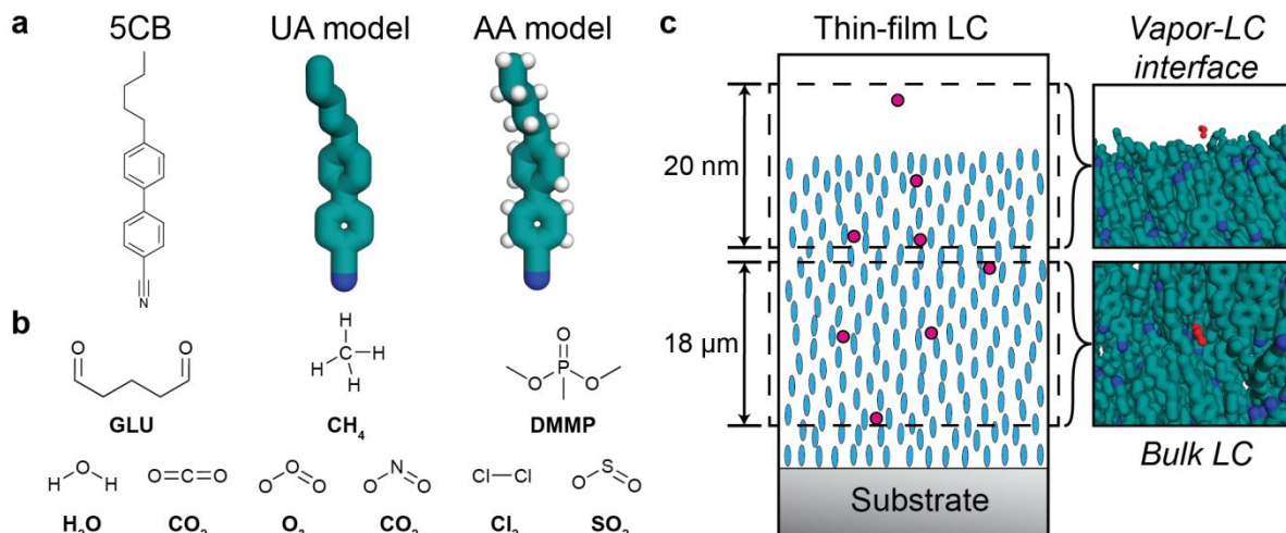
Figure 1: Overview of simulation systems. a) Chemical structure of 5CB and snapshots of UA and AA simulation representations. b) Chemical structures of all analytes considered. c) Schematic of a chemoresponsive liquid crystal (LC) sensor prior to sensor activation. Blue ellipsoids indicate the mesogens in a nematic phase. Red circles illustrate the partitioning and diffusion of analytes toward the substrate. Snapshots of simulation systems representative of the vapor-LC interface and bulk nematic LC are shown at right.
