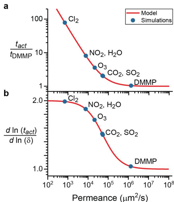
Figure 6: Mass-transport model of sensor activation. a) Relative response time as a function of permeance for all six analytes. Response times are calculated relative to the response time for DMMP, which was experimentally measured to be between 10 and 100 s. b) The leading order polynomial dependence of the response time on film thickness as a function of permeance for all six analytes.
