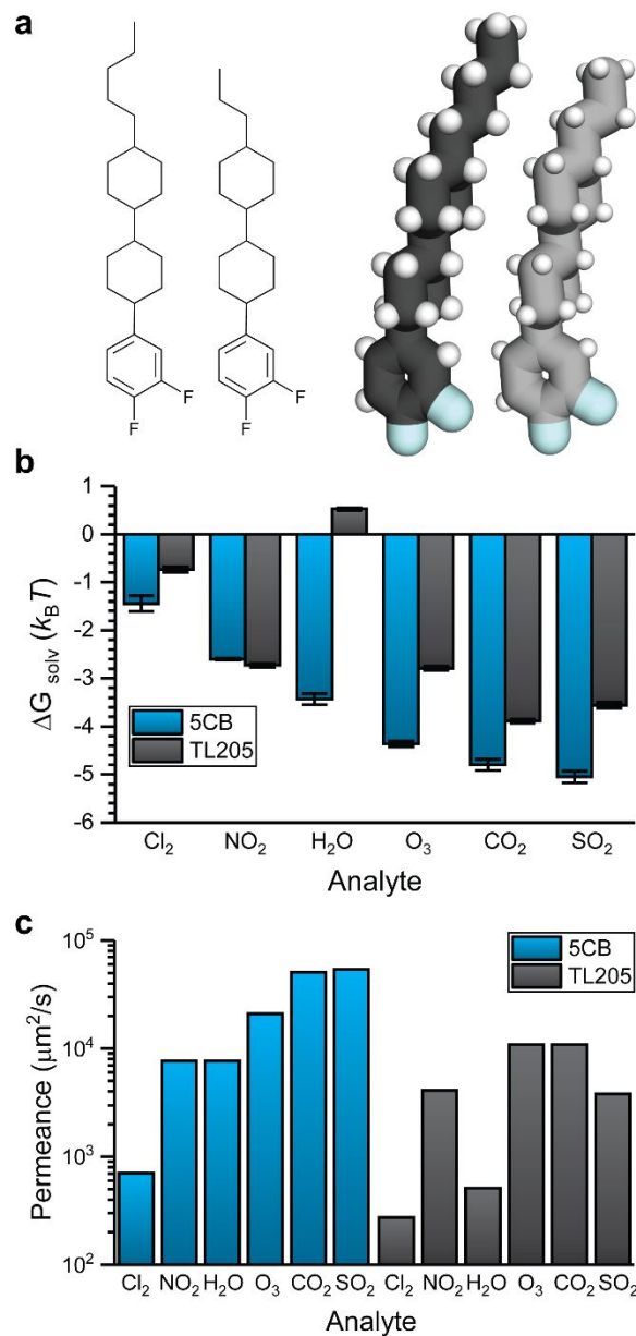
Figure 7: Analyte partitioning and transport in TL205. a) Chemical structures and simulation snapshots of two components used to represent the mesogen mixture in TL205. b) Comparison of solvation free energies for all analytes in 5CB and in TL205. c) Comparison of permeances for all analytes in 5CB and TL205.
