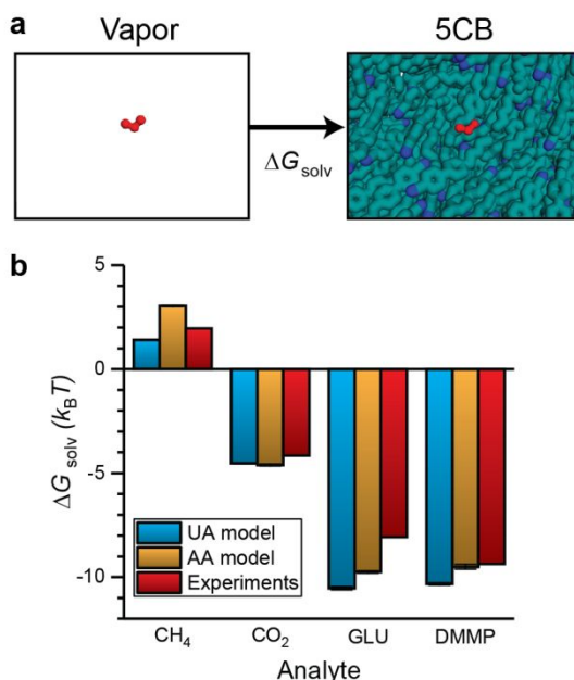
Figure 3: Validation of solvation free energy calculations. a) Simulation snapshots illustrating the two states used to calculate the solvation free energy ( \Delta G_{\text{solv}} ). The analyte is shown in red. b) \Delta G_{\text{solv}} calculated using the UA and AA 5CB models. Values are compared to experimental estimates based on Henry's law constants using Equation 2.
