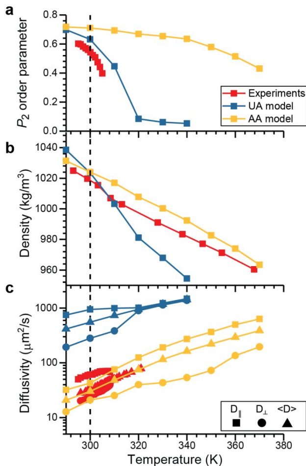
Figure 2: Comparison of 5CB model predictions to experimental measurements. All plots compare the temperature dependence of a bulk 5CB property calculated using either the UA (blue) or AA (yellow) model to experimental measurements (red). Squares indicate the temperatures at which simulations/experiments were performed. A dashed line is drawn at 300 K as a guide to the eye. Properties include: (a) the P_2 order parameter, with experimental data from Ref. 56 ; (b) the bulk density, with experimental data from Ref. 57 ; and (c) 5CB diffusion coefficients, with experimental data from Ref. 58 . The component of the diffusion coefficient parallel to the director vector ( D_{\parallel} ), the component perpendicular to the director vector ( D_{\perp} ), and the average diffusion coefficient ( \langle D \rangle ) are separately reported.
