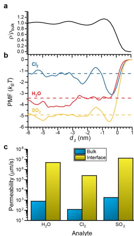
Figure 5: Comparison of bulk and interfacial partitioning. a) 5CB density as a function of the z -component of the distance from the vapor-LC interface ( d_z ). The density is normalized by the density of bulk 5CB in the nematic phase. b) Potentials of mean force (PMFs) as a function of d_z for \text{Cl}_2 , \text{H}_2\text{O} , and \text{SO}_2 . PMF values are set to zero at d_z = 1 nm. c) Permeabilities computed for the bulk LC and the interfacial region using Equation 4.
