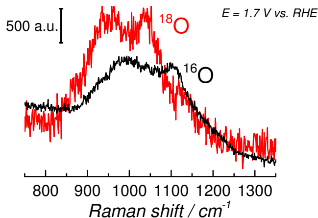
Figure 3. SER spectra of NiOOH in the wavenumber region 800 – 1350 cm -1 . The spectra were obtained at 1.7 V vs. RHE in Na 16 OH 0.1 M. The electrolyte was prepared with H 2 16 O and H 2 18 O.
