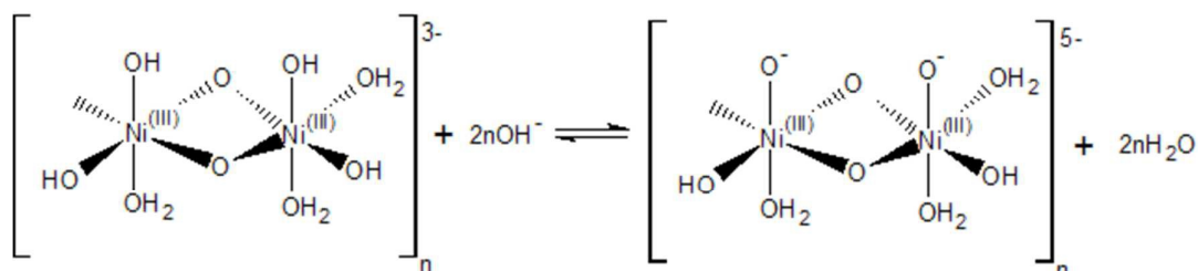
Scheme 2. Hydroxide-mediated deprotonation process of the surface of \text{NiO}(\text{OH}) towards negatively charged species.
