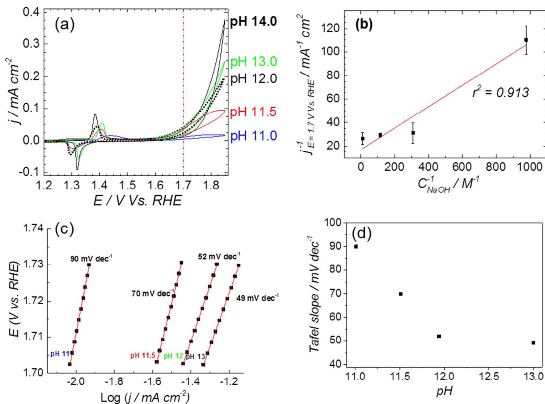
Figure 1. (a) CVs of NiOOH deposited on Au, showing the Ni II / Ni III redox peaks and the OER activity at E > 1.65 V. Measurements at pH 11 – 13 were performed at constant ionic strength, adjusted to 0.1 M with NaClO 4 except for pH 13 and pH 14, those solutions solution were NaOH 0.1 M and 1 M, respectively. Scan rate: 0.01 V/s. (b) Langmuir-type plot of the OER activity as a function of the concentration of NaOH in the electrolyte (pH 11 – 13), the activity was measured from the CV's as the average of the backwards and forward current density at 1.7 V vs. RHE (red dashed line in a)). (c) Tafel plot, obtained from the CV's in (a) as the average of the backwards and forward current density in the potential region 1.702-1.73 V vs. RHE. (d) Tafel slope as a function of the electrolyte pH.
