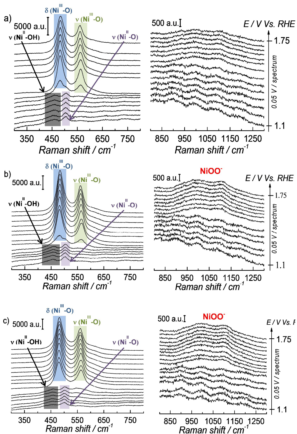
Figure 2. SER spectra obtained at constant potential during the electrochemical oxidation of \text{Ni}(\text{OH})_2 and the subsequent OER on \text{NiOOH} at different pH's. The ionic strength of the solution was fixed to 0.1 M with \text{NaClO}_4 except for pH 13, that solution is \text{NaOH} 0.1 M. The left panel presents the spectra in the wavenumber region 300 – 800 \text{cm}^{-1} and the right panel presents the wavenumber region 800 – 1300 \text{cm}^{-1} : a) pH 11, b) pH 12.0, c) pH 13.0.
