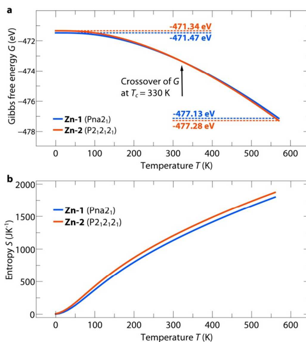
Figure 2. Temperature dependence of the Gibbs free energy G (a) and entropy S (b) of the compounds Zn-1 (blue) and Zn-2 (orange). With increasing temperature, the entropic contribution becomes more dominant which causes the crossover of G at T_c = 330 K. The higher vibrational entropy of the channel structure is caused by a lower density and weaker hydrogen bonding pattern.
