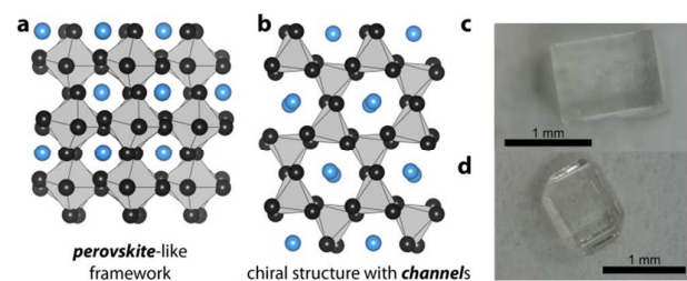
Figure 1. Schematics of the two structure types observed in the series [\text{NH}_3\text{NH}_2]\text{B}(\text{HCOO})_3 with \text{B} = \text{Mn}^{2+} , \text{Co}^{2+} , \text{Zn}^{2+} and \text{Mg}^{2+} . The structures are simplified to emphasize the perovskite-structure motif in (a) and the hexagonal channels in (b). Grey polyhedrons are \text{ZnO}_6 octahedrons, black spheres formate anions and blue spheres correspond to [\text{NH}_3\text{NH}_2]^+ cations. (c) and (d) show crystals of Zn-1 (c) and Zn-2 (d), see ESI for more crystals.
