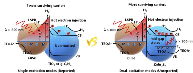
Fig. 4 Schematic of the newly developed plasmon-mediated photocatalysts using the earth-abundant copper chalcogenide (CuSe) for NIR-driven photocatalytic H_2 production. A possible band diagram and NIR-induced carrier dynamics in the plasmonic heterojunction are shown, illustrating the NIR light-driven photocatalytic reaction ( E_U : the energy of the band tail, also referred to as the Urbach energy).
