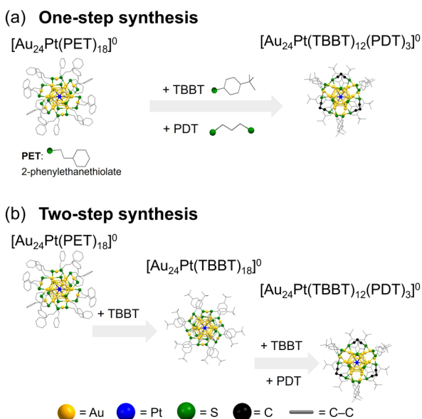
Fig. 2 Schematic of the (a) one-step and (b) two-step synthetic methods for preparing [Au_{24}Pt(TBBT)_{12}(PDT)_3]^0 from [Au_{24}Pt(PET)_{18}]^0 .
