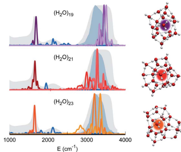
Fig. 3 Power spectra of the central monomer. The peaks corresponding to bending (darker color nuances), stretching (lighter color nuances), and most coupled bending–libration modes (blue) of (\text{H}_2\text{O})_{19} (top), (\text{H}_2\text{O})_{21} (middle), and (\text{H}_2\text{O})_{23} (bottom) are reported. The liquid water IR spectrum is shown as shaded gray areas, and the MCR-Raman band (from ref. 75) for the stretching of tetrahedrally coordinated monomers in liquid water (light blue) is also presented. Reproduced from A. Rognoni, R. Conte and M. Ceotto, Chem. Sci. , 2021, 12, 2060–2064.
