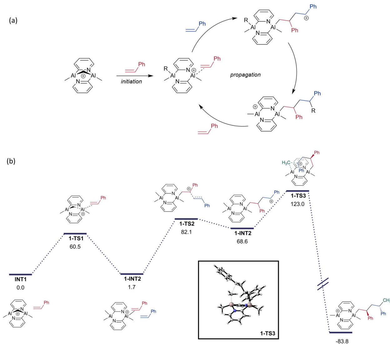
Fig. 9 (a) Viable mechanism involving dimer transfer, and (b) energy profile of the dimer transfer-based polymerisation mechanism (Gibbs free energies in \text{kJ mol}^{-1} ). The TS for the S_E2 (back) reaction is highlighted in the box.
