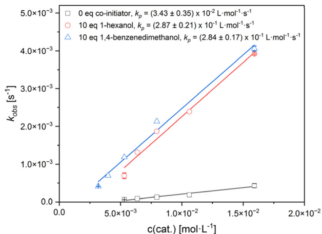
Fig. 4 Determination of the reaction rate constant k_p of ROP of L-lactide with C1 and 10 eq. 1-hexanol (Co11, red circles) and 1,4-benzenedimethanol (Co12, blue triangles), or without co-initiator (black squares) by plotting the apparent rate coefficient k_{\text{obs}} from the initial ranges over the catalyst concentration.
