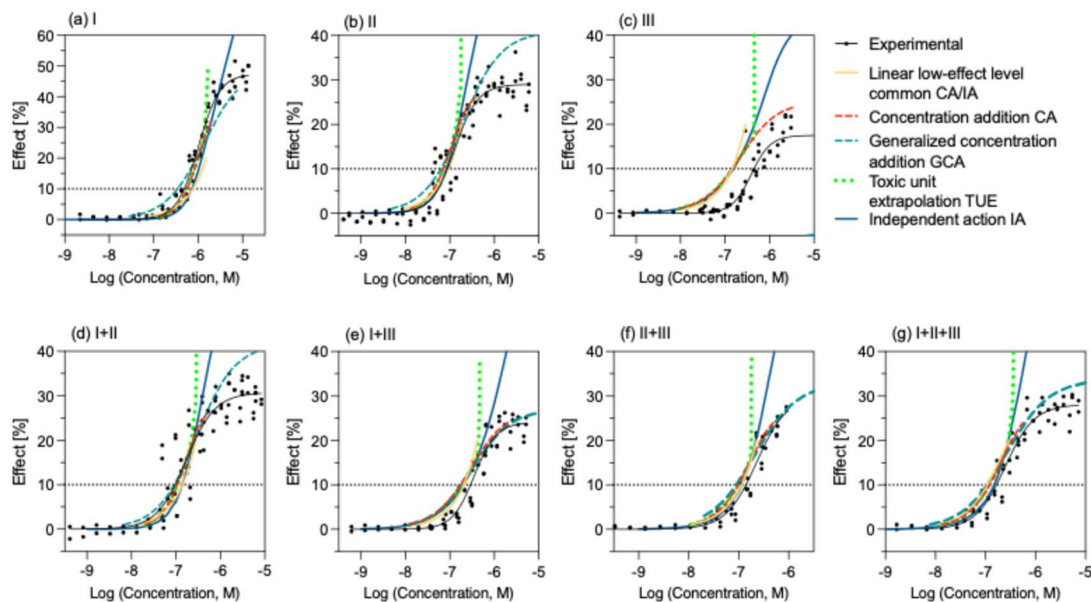
Fig. 3 Full concentration–effect curves for estrogen receptor ER\alpha activation in ER\alpha -UAS-bla GripTite. (a) Mixtures I, (b) II, (c) III, (d) I + II, (e) I + III, (f) II + III, (g) I + II + III. Black dots are the experimental data points and black thin line fit with the full-range log-logistic model (eqn (5)). Linear CA&IA (mango line) refers to the linear low-effect model for prediction of concentration addition (CA)/independent action (IA) (eqn (10)). CA (red dashed line) prediction with eqn (6) from the full log-logistic CRC of the single chemicals; IA (blue solid line) refers to IA prediction with eqn (7) from the full log-logistic CRC of the single chemicals; GCA (dashed teal line) refers to general concentration addition model (eqn (11)) and TUE (light green dotted line) to toxic unit extrapolation model (eqn (14)). All data from Table S7.
