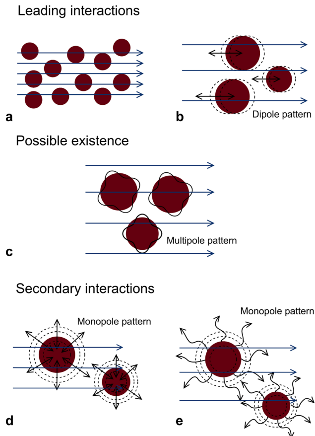
Fig. 9 Leading interaction mechanisms between ultrasonic waves and a suspended particle in a concentrated slurry. 40 (a) Material substitution; (b) density contrast; (c) multipole particle resonance (strong when incident wave length matches resonance). Secondary mechanisms: (d) compressibility contrast; (e) thermal contrast.
