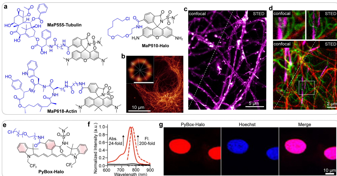
Fig. 23 (a) Chemical structures of various MaP labels. (b) Wash-free STED imaging of microtubules in live U2OS cells labelled with MaP555-tubulin. Scale bar: 10 \mu\text{m} . Inset shows the deconvoluted image of a selected centriole, with dotted lines indicating the nine intensity maxima corresponding to the nine microtubule triples. Scale bar: 200 nm. (c) Wash-free confocal and STED images revealing periodic actin structures in the axons of rat primary hippocampal neurons labeled with MaP618-actin. Scale bar: 5 \mu\text{m} . (d) No-wash three-color confocal and STED images of live U2OS Vimentin-Halo-expressing cells stained with MaP510-Halo (green), MaP555-tubulin (red), MaP618-actin (magenta), and verapamil for 2 h. The top panels show magnified confocal and STED images of the region indicated by the white box in the bottom panel. Image data were smoothed using a one-pixel Gaussian low-pass filter. Scale bar: 2 \mu\text{m} . (e) Chemical structure of PyBox-Halo label. (f) Absorption (solid line) and fluorescence (dashed line) spectra of PyBox-Halo (black) and PyBox-Halo with HaloTag7 (red) in pH 7.3 HEPES buffer. (g) No-wash live-cell confocal images of U-2 OS cells expressing HaloTag-histone H2B labeled with PyBox-Halo. Scale bars: 10 \mu\text{m} . (b)–(d), (f) and (g) are adapted from ref. 139 and 149 with permission from Springer Nature and the American Chemical Society, copyright 2020 and 2023, respectively.
