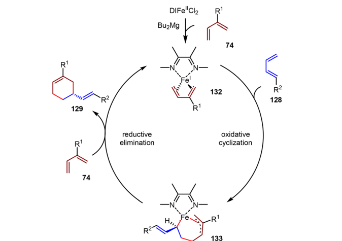
Scheme 29 Fe(I)/ \alpha -diimine-catalyzed asymmetric cross-[4+2] cycloadditions of unactivated 1,3-dienes.
