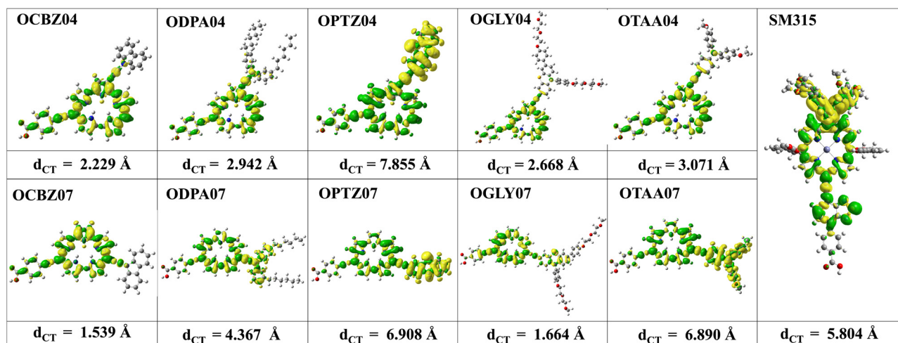
Fig. 6 Plot showing the charge density difference (CDD) and charge transfer distance ( d_{CT} ), calculated at the MN15/6-311+G(d,p) level of theory. Here, yellow zones represent electron-rich regions and green zones represent electron-deficient regions. An iso-contour value of 0.0004 a.u. was used for the d_{CT} plot.
